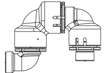
STYLE 800 Three-Ell Triple Swivel
